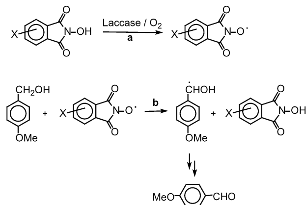
Scheme 5 Mechanism of oxidation of p -anisyl alcohol promoted by laccase/X-HPI/ O_2 systems.
