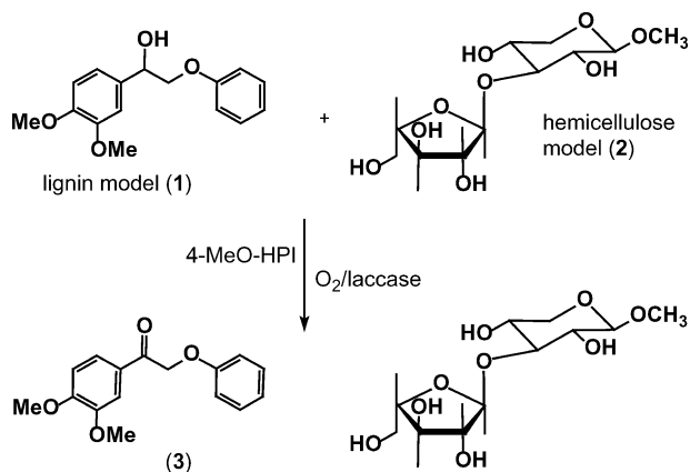
Scheme 6 Competitive oxidation of a lignin model (1) and of a polysaccharide model (2).
