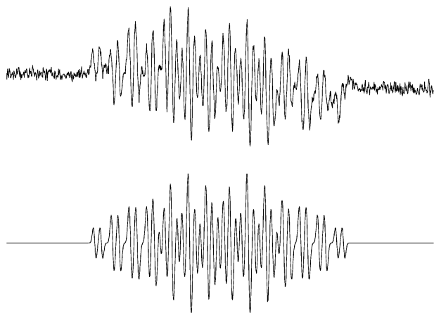
Fig. 2 Experimental EPR spectrum from HBO with CAN in MeCN (upper) and its computer simulation (lower); EPR data: a(\text{N}) = 1.38 \text{ G} , a(\text{N}) = 2.74 \text{ G} , a(\text{N}) = 4.60 \text{ G} ; a(\text{H}) = 0.53 \text{ G} , a(\text{H}) = 1.38 \text{ G} ; g = 2.0062 .
