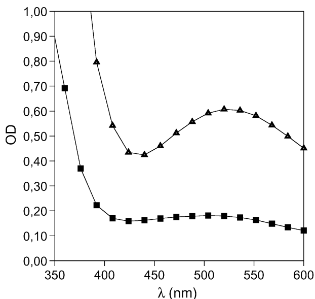
Fig. 1 UV-Vis spectrum of BONO in MeCN: (a) immediately after the generation with CAN (curve ▲), (b) after 2 h (curve ■).
