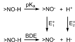
Scheme 8 Thermochemical cycle for determining \text{BDE}_{\text{NO-H}} values.
