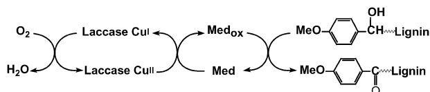
Scheme 1 The oxidation cycle of a laccase/mediator system towards non-phenolic substrates.
