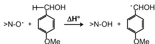
Scheme 3 The thermochemical scheme of the radical H-atom transfer (HAT) mechanism between a >N–O • species and a C–H donor substrate.
