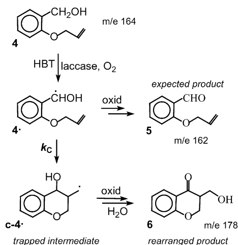
Scheme 7 Intercepting the radical intermediate of the HAT oxidation mechanism.
